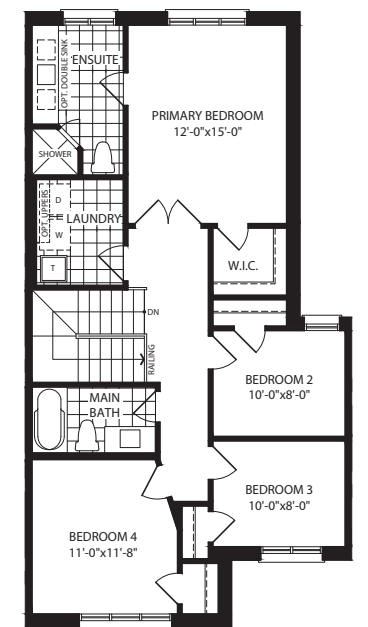
OPTIONAL SECOND FLOOR A 4 BEDROOM
