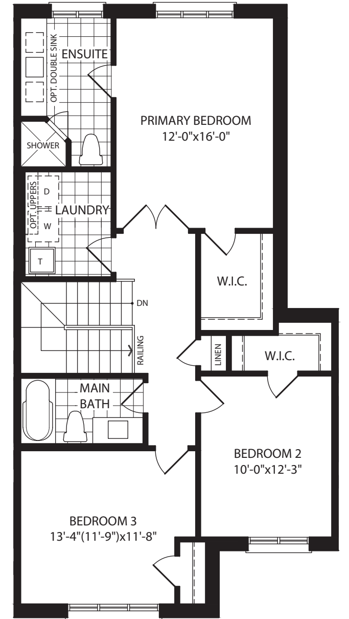
SECOND FLOOR A
