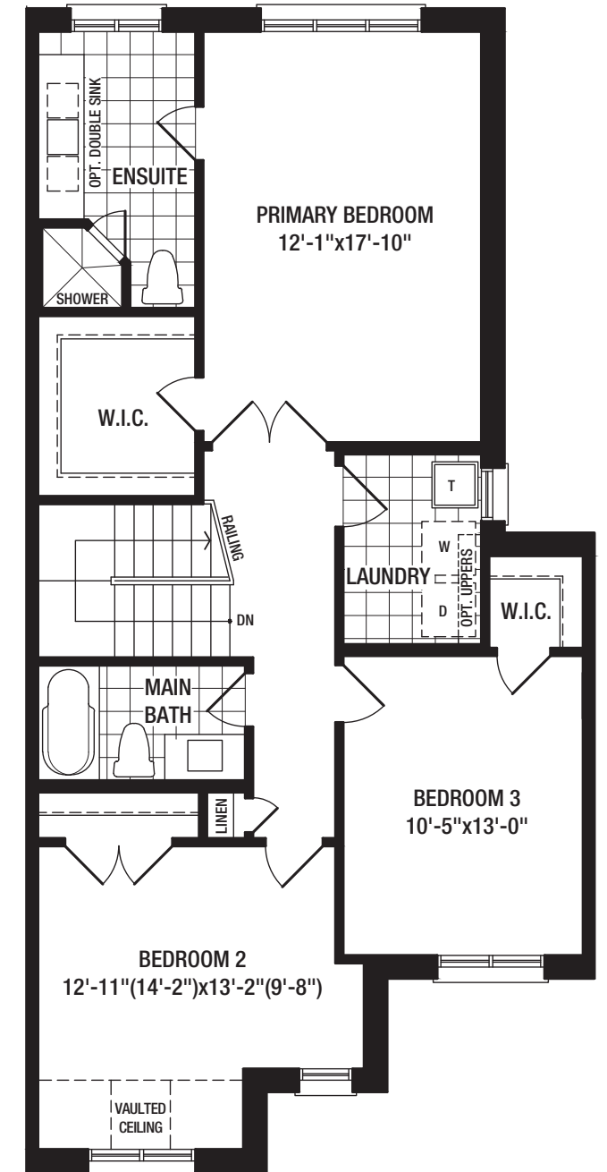
SECOND FLOOR A
