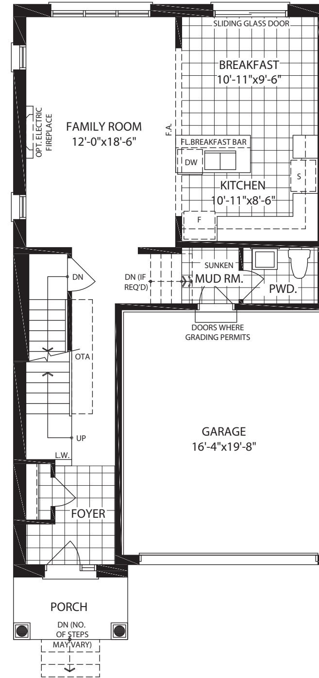
MAIN FLOOR A
