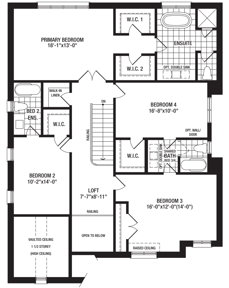
SECOND FLOOR A
