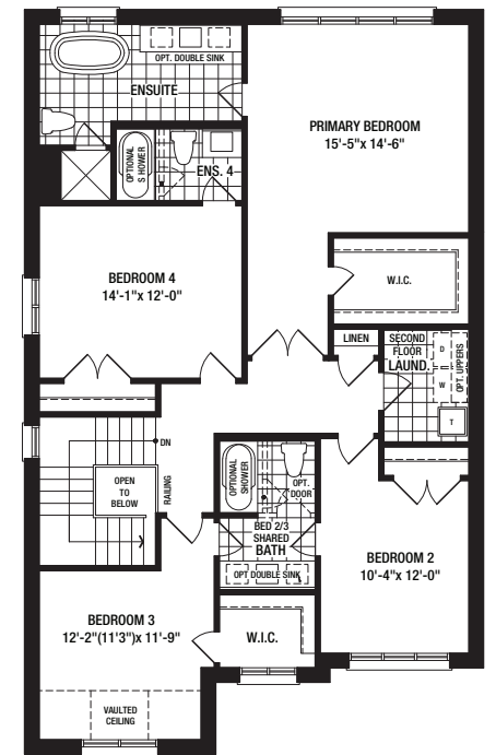
OPTIONAL SECOND FLOOR A 4 BEDROOM
