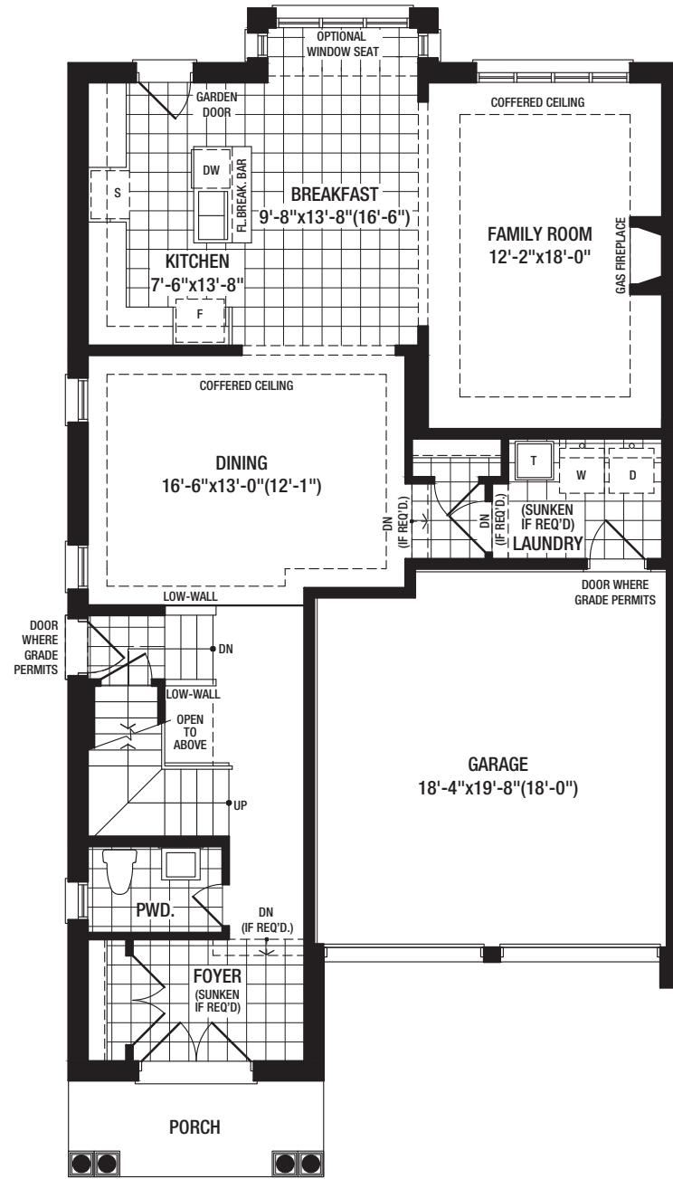
MAIN FLOOR A
