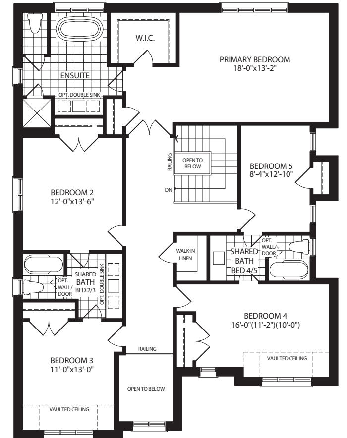
OPTIONAL SECOND FLOOR A - 5 BEDROOM
