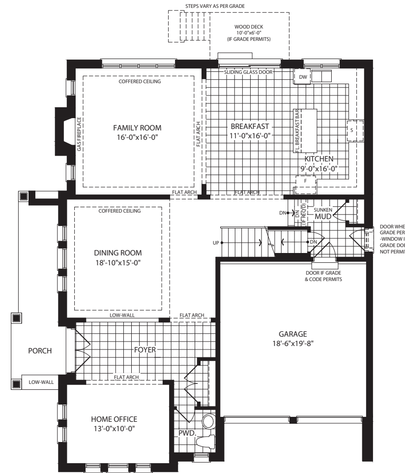
MAIN FLOOR A
