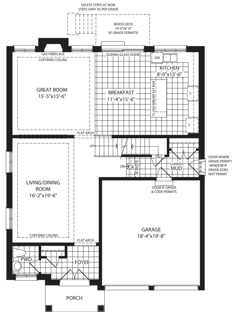
MAIN FLOOR A
