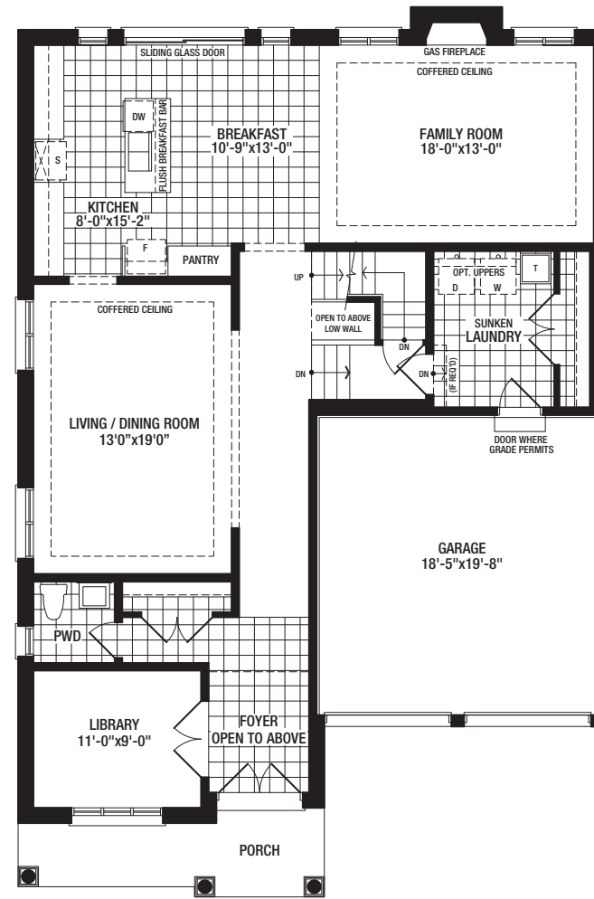
MAIN FLOOR A
